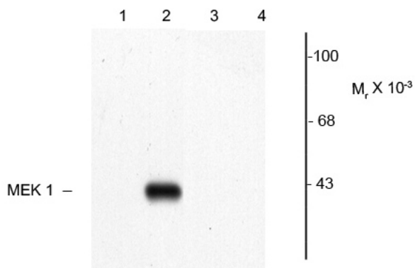
ARG52334 anti-MEK1 phospho (Thr292) antibody WB image
