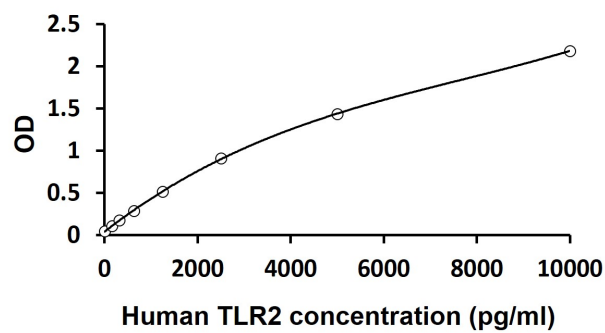
ARG81475 Human TLR2 ELISA Kit standard curve image
