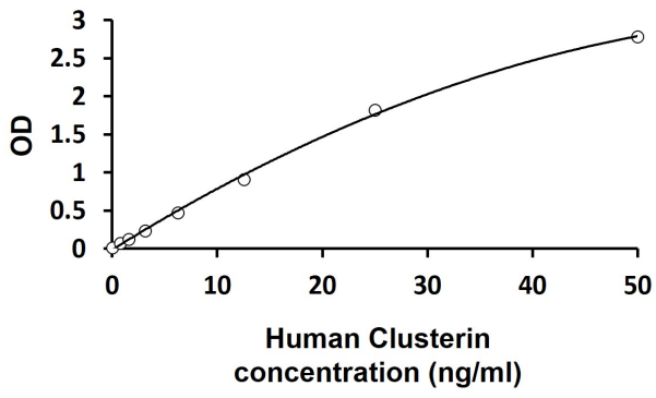
ARG81479 Human ApoJ / Clusterin ELISA Kit standard curve image
