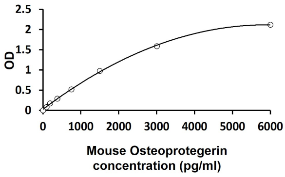
ARG81667 Mouse TNFRSF11B / OPG ELISA Kit standard curve image
