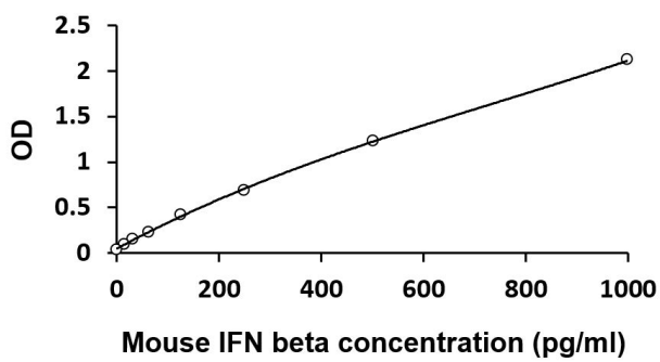
ARG82317 Mouse IFN beta ELISA Kit standard curve image
