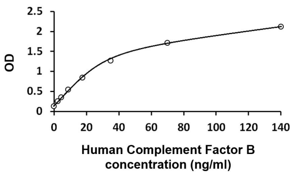
ARG82648 Human Complement Factor B ELISA Kit standard curve image
