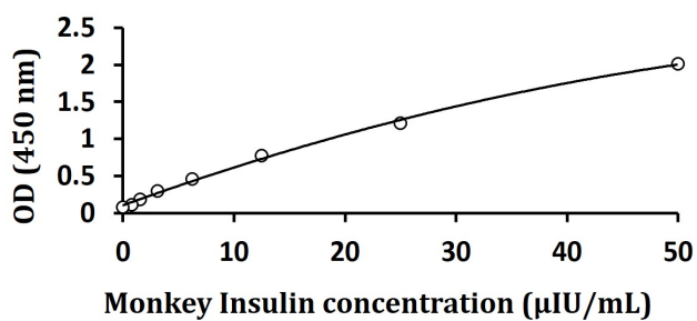
ARG82671 Monkey Insulin ELISA Kit standard curve image
